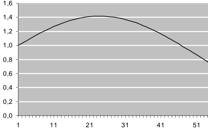
Figure 1. Deterministic age-dependent productivity term, \widehat{e}_j .
